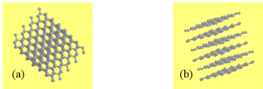
Figure 1. (a) Diamond structure and (b) graphite's layered structure [12].
