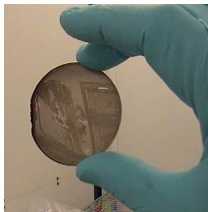
Figure 2. Free standing polycrystalline diamond, ~50 mm diameter and ~230 μm thick.
